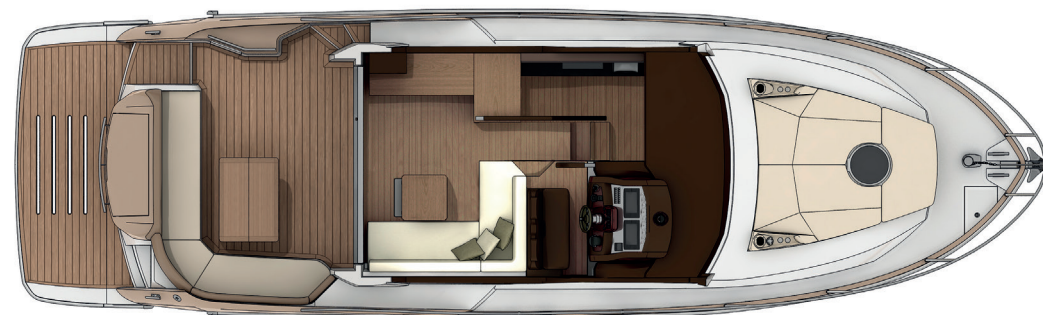
MAIN DECK
